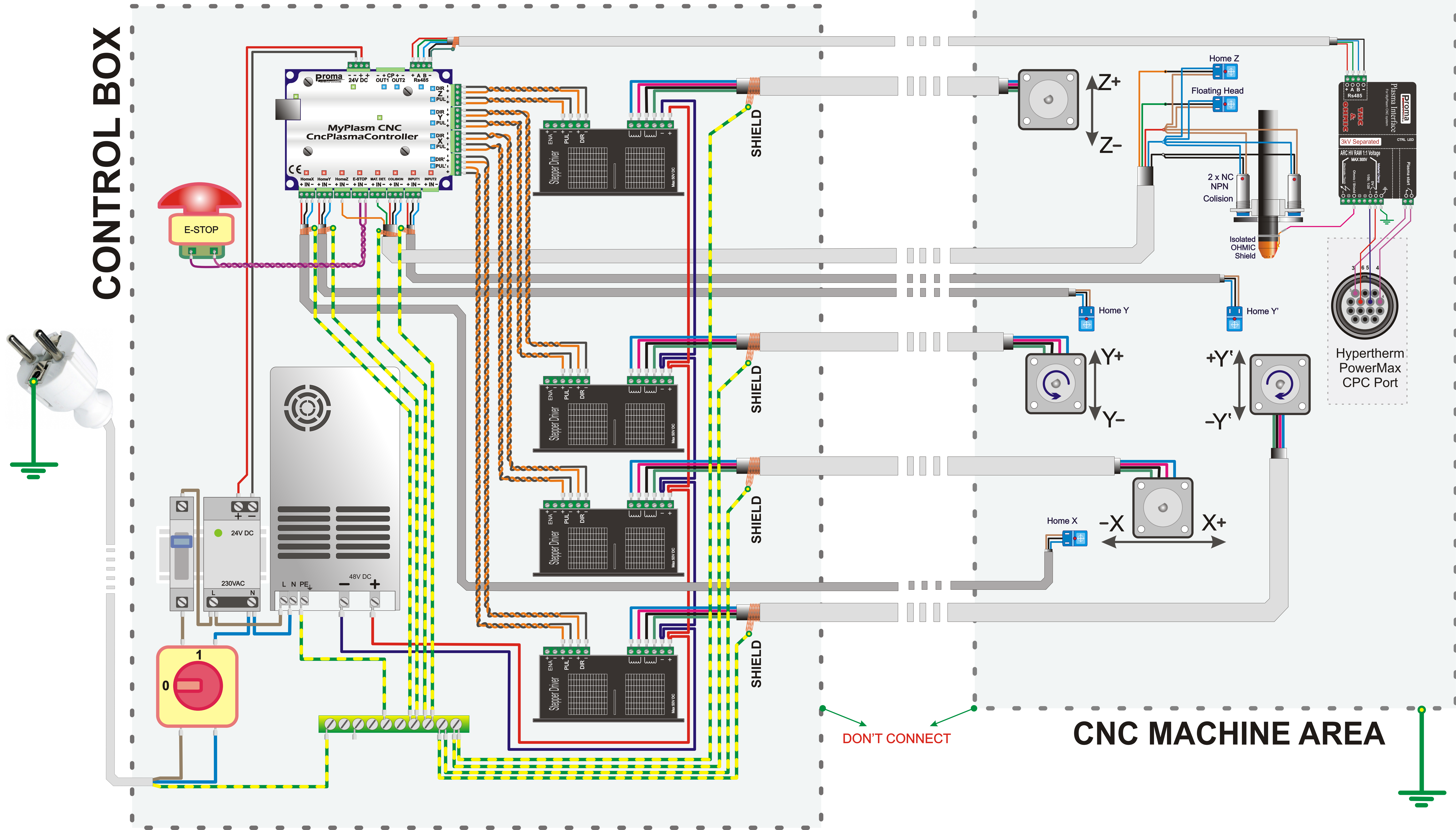
Example of SYSTEM connections
